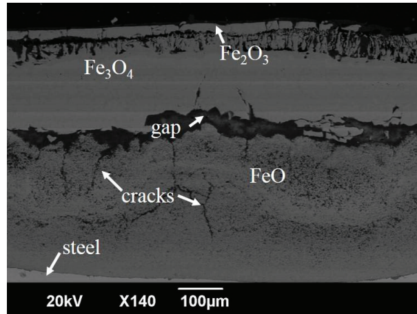
FIGURE 5. SEM of cross sectional morphology of SAPH440 oxidized at 750 °C for 49 h in the burning ethanol atmosphere
