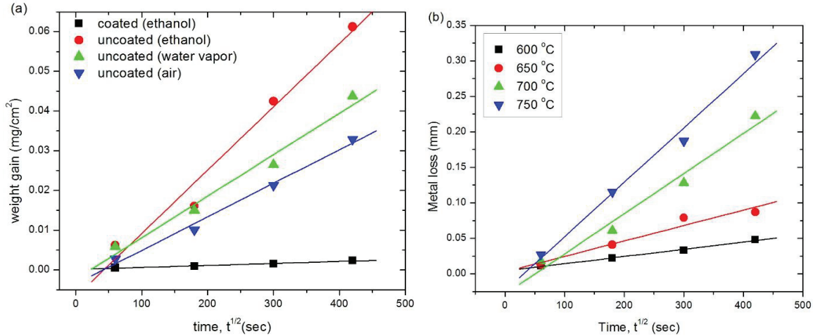
FIGURE 1. (a) The parabolic plot of weight gain curves of the specimens being oxidized at 750^\circ\text{C} for 49 h, (b) metal loss vs. the square root of the time the bare steel was exposed to the burning ethanol atmosphere at an elevated temperature.
