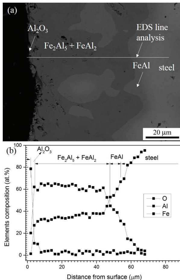
FIGURE 2. (a) SEM morphology of a cross-sectional image and (b) EDS line profile of the aluminized steel after oxidation in the burning ethanol atmosphere at 700 °C for 25 h
