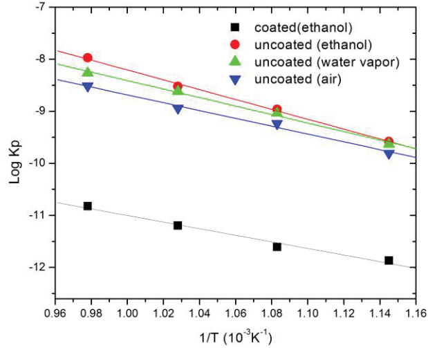
FIGURE 4. Relationship between \log k_p and 1/T for the SAPH440 steel under isothermal oxidation conditions in the different atmospheres
