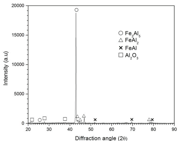
FIGURE 3. X-RD diffraction patterns of the aluminized steel after oxidation in a burning ethanol atmosphere at 700 °C for 49 h
