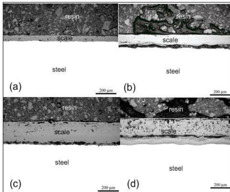
FIGURE 6. Cross-sectional morphologies of SAPH440 steel oxidized at (a) 600 °C, (b) 650 °C, (c) 700 °C, and (d) 750 °C for 25 h in a burning ethanol atmosphere
