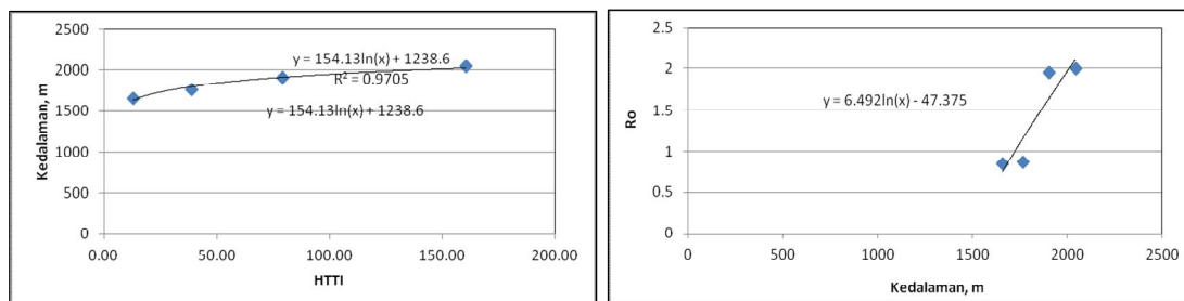
Figure 2. Graph depth against HTTI and Ro Well BGS-1
