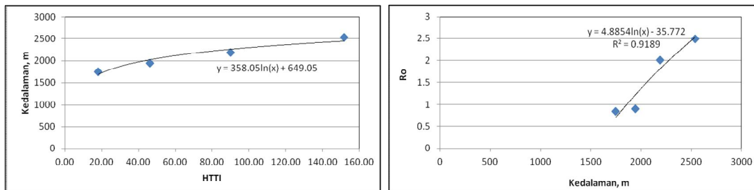
Figure 5. Graph depth against HTTI and Ro Wells BGS-4
