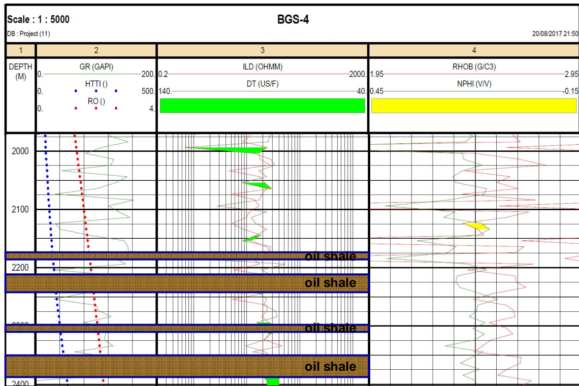
Figure 10. Plot Log Chart HTTI-Ro-GR, Sonic-Lld, NPHI-RHOB Wells BGS-4
