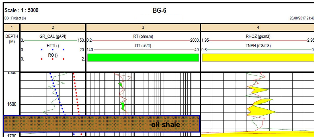
Figure 6. Graph HTTI Log-Ro-GR, Sonic-Lld, NPHI-RHOB Well BG-6
