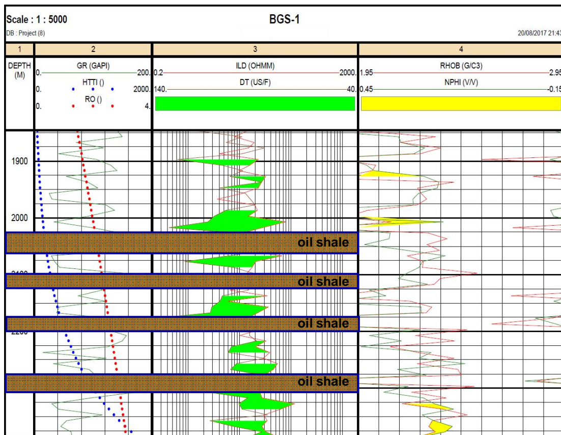
Figure 7. Graph HTTI Log-Ro-GR, Sonic-Lld, NPHI-RHOB Well BGS-1
