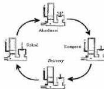
Gambar 1. Siklus kerja pompa hydram (Silvers, 1977)
