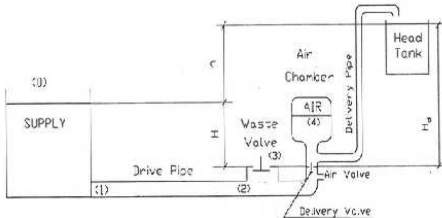
Gambar 2. Skema instalasi pompa hydrum ( Taye, 1998)
