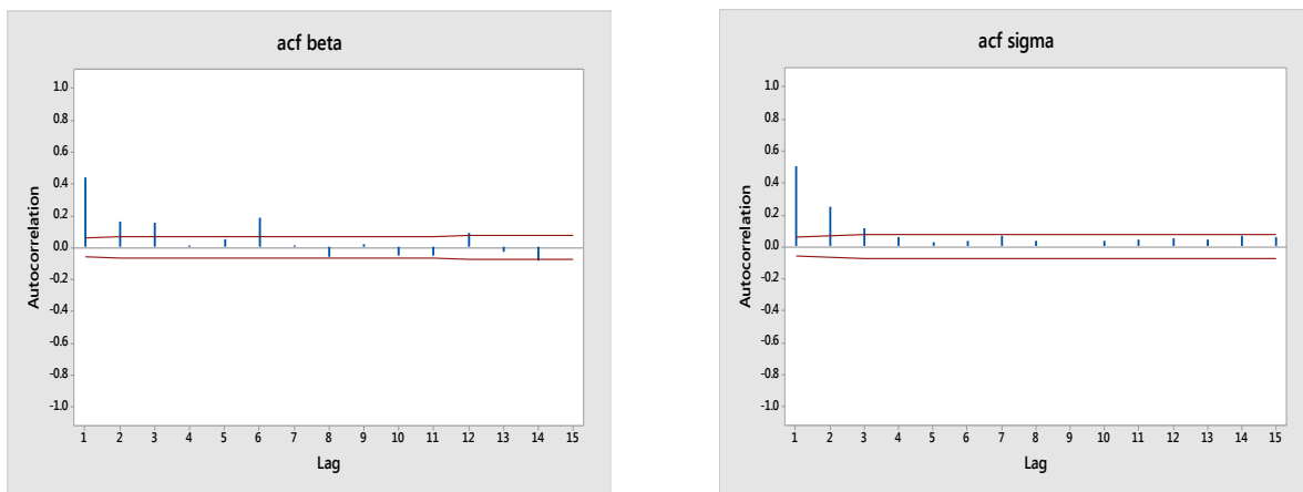
Fig. 4. Autocorrelation Function Plot for Beta and Sigma Parameter
