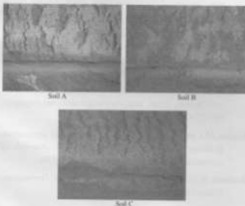
Figure 6. Horizontally cutting mole in soil A, B, and C
