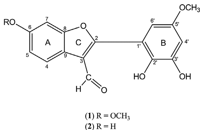
Figure 1. The structures of the isolated compounds.
