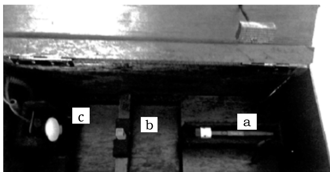
Figure 1. Photograph of the photometer apparatus: (a) green laser pointer, (b) sample holder, (c) lux meter.
