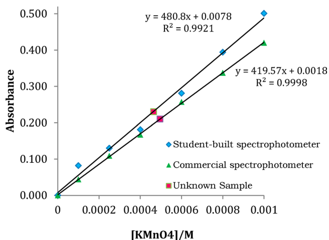
Figure 5. Calibration curve for a series of standard potassium permanganate solutions from two types of instruments. All measurements were made with a 1 cm path cell. Deviation of the mean (DM) for the student-built photometer = 0.0045; DM for the commercial HSP 788 UV-vis spectrophotometer = 0.0009.
