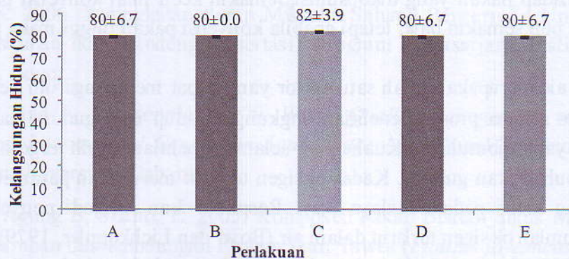
Gambar 4. Survival rate
