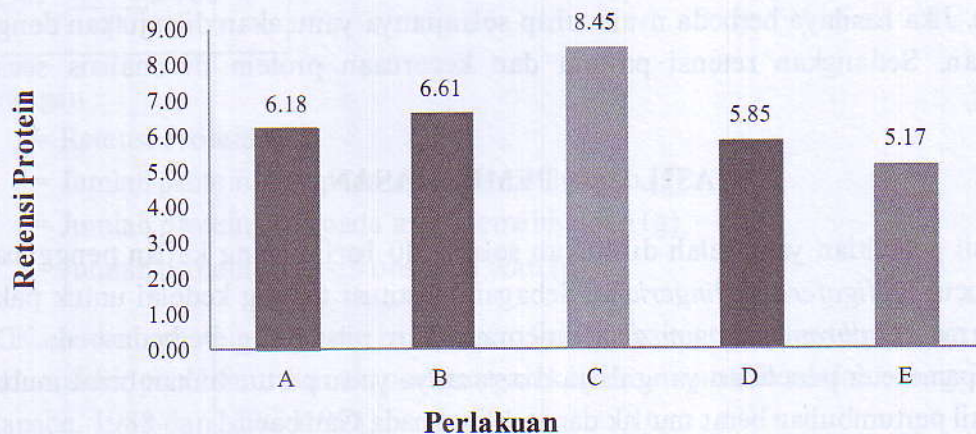
Gambar 2. Retensi protein
