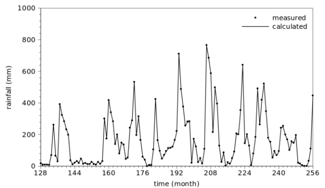
Fig. 10. Variation of measured and calculated periodic + stochastic monthly rainfall from station Purajaya (128-256).
