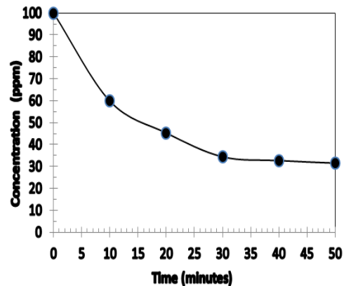
Figure 6. The effect of UV light irradiation exposure time on the concentration of methanyl yellow azo-dye in the sample
