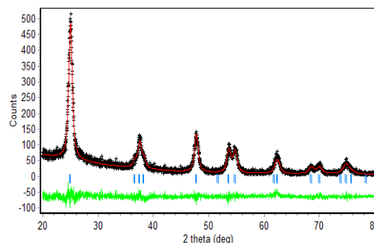
Figure 2. Quantitative analysis of Si doped TiO 2 diffractogram fitted using Rietveld method. The observed and the calculated data are shown by the (+) black and red signs, respectively. The blue strips (below) refers to point series of hkl and the green line is the difference profile between observed and calculated data.
