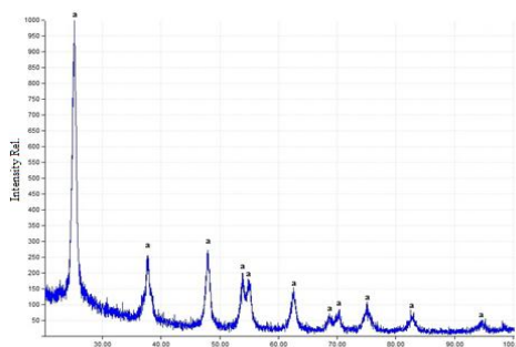
Figure 1. Diffractogram S-doped TiO 2 (with 0.02 mole of sulphur; and a = anatase phase) and calcined at 400°C
