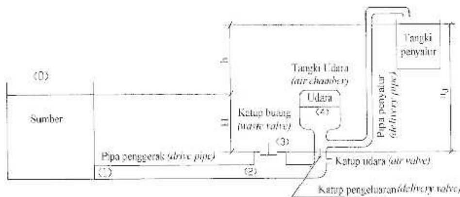
Gambar 1. Instalasi pompa hydraulic ram pump
