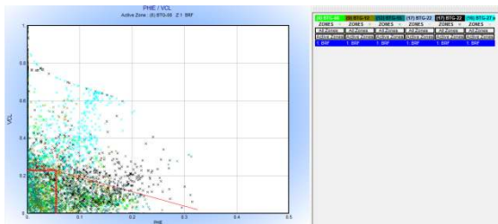
Gambar 18. Penentuan Cutoff Volume Clay ( V_{cl} )
