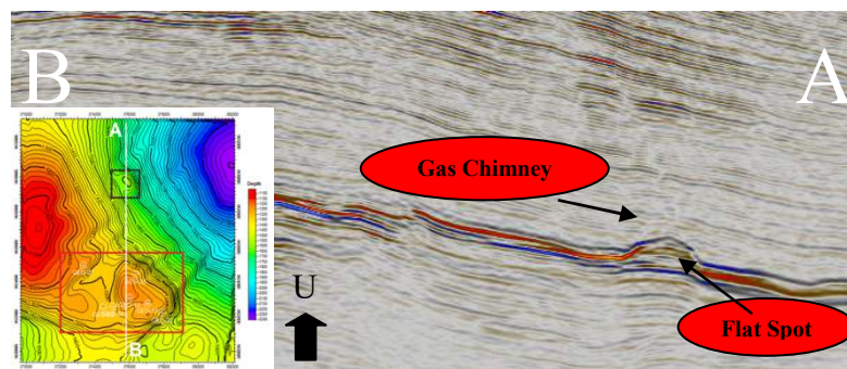
Gambar 10. Analisis DHI Fokus Area Outstep
