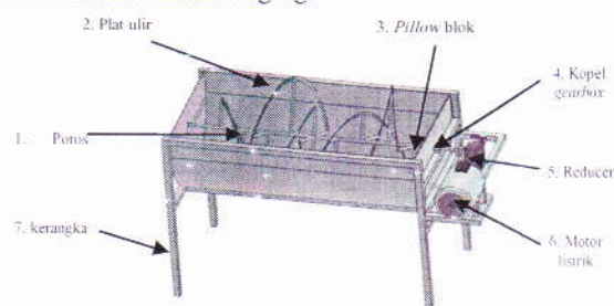
Gambar 1. Disain alat mesin mixer bahan baglog
