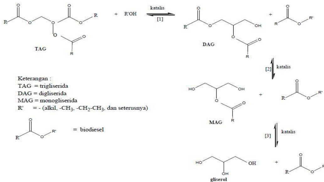
Fig. 10. The mechanism of transesterification reaction with base catalyst (Singh,2010)
