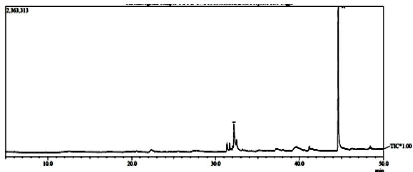
Fig. 12. GC-MS result for Tetraselmis chuii FAME
