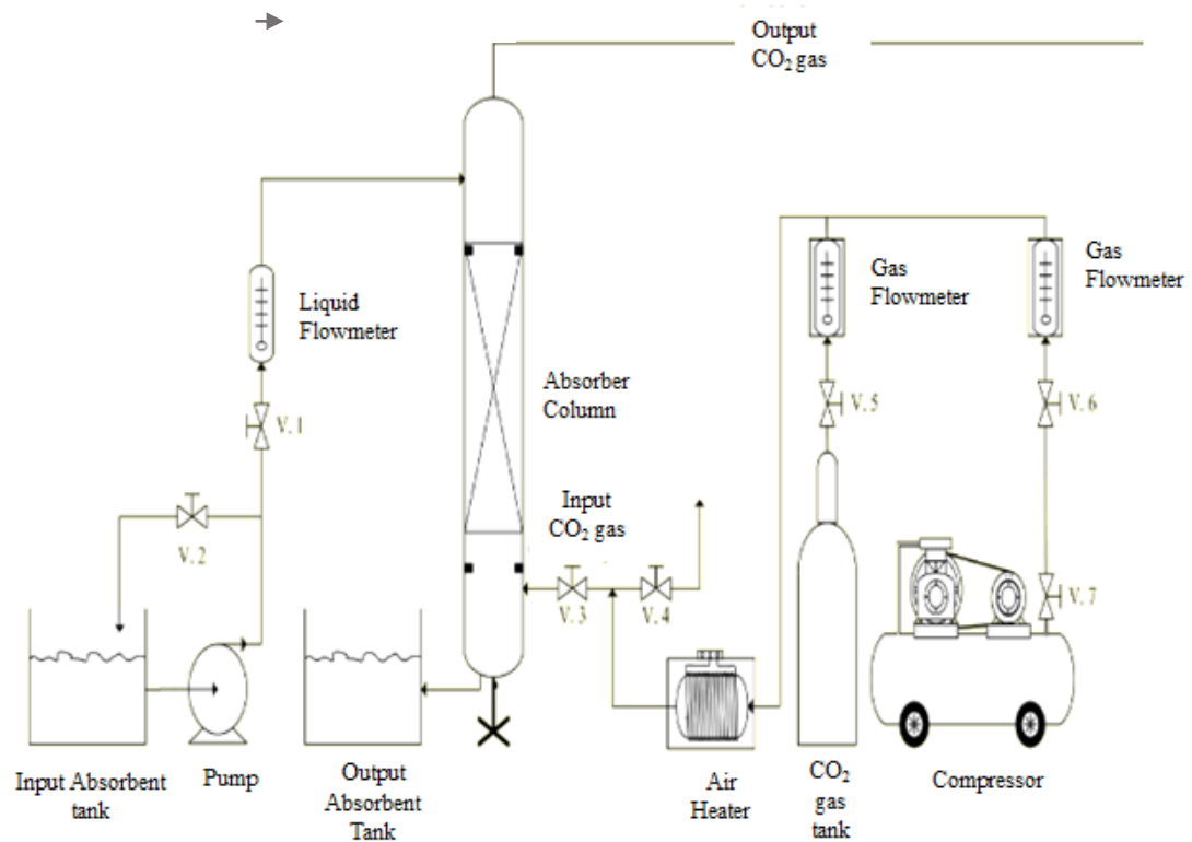
Fig. 1. Schematic of CO 2 absorption tool setting
