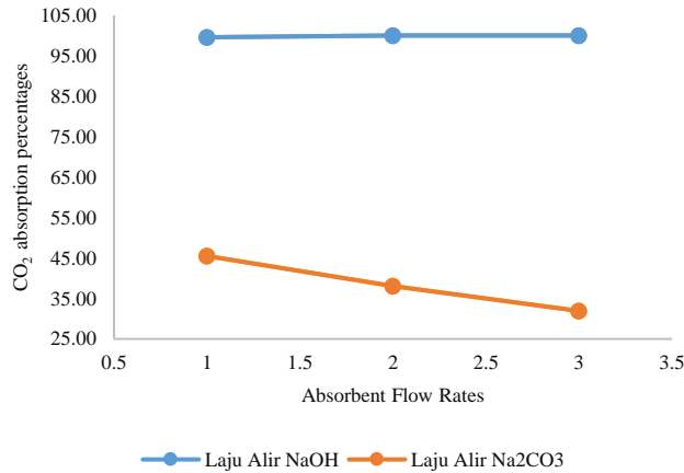
Figure 4. The effect of flow rates on the percentage of CO 2 absorption
