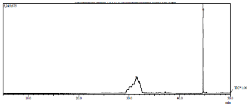
Fig. 11. GC-MS result for Nannochloropsis oculata FAME
