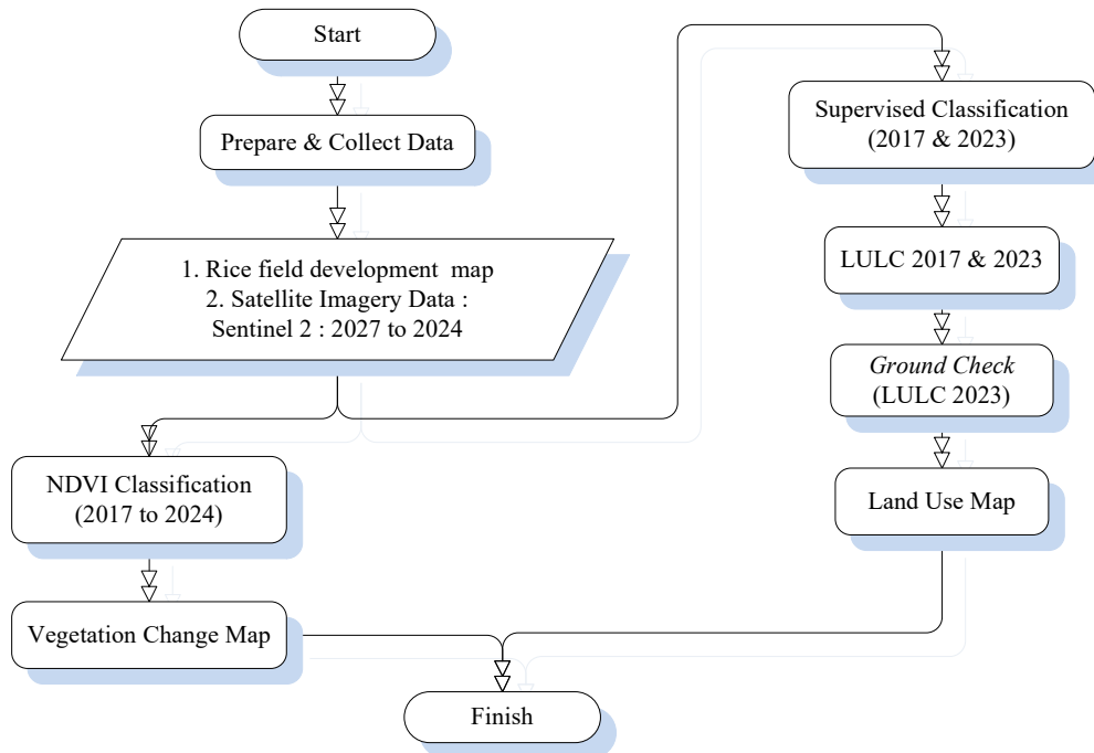
Gambar 2. Flowchart Penelitian
