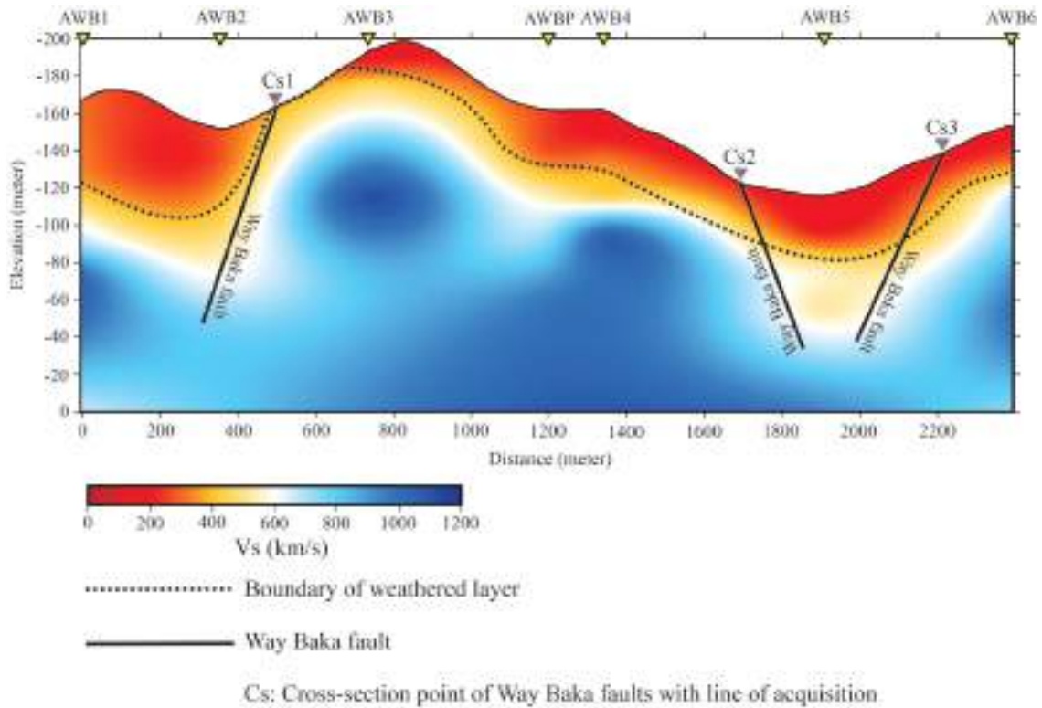
Figure 8. The interpretation of the Way Baka Fault existence in 2D cross-section of microtremor data inversion results at the study site. The yellow triangle with the AWB label indicates the microtremor measurement point, while the gray triangle with the Cs label indicates the intersection point with the fault.
