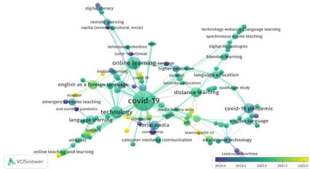
Fig. 5. Overlay visualization of co-word analysis.
