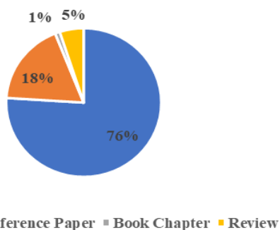
Fig. 2. Total papers by document type.
