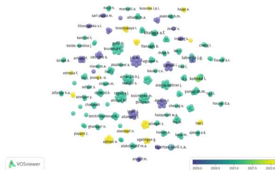
Fig. 7. Overlay visualization of co-author analysis.
