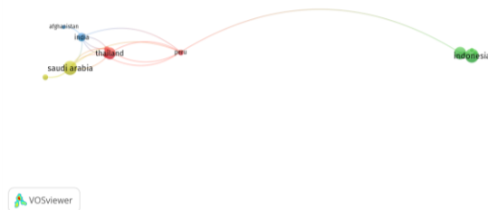
Fig. 8. Network visualization of co-author analysis in country unit.
