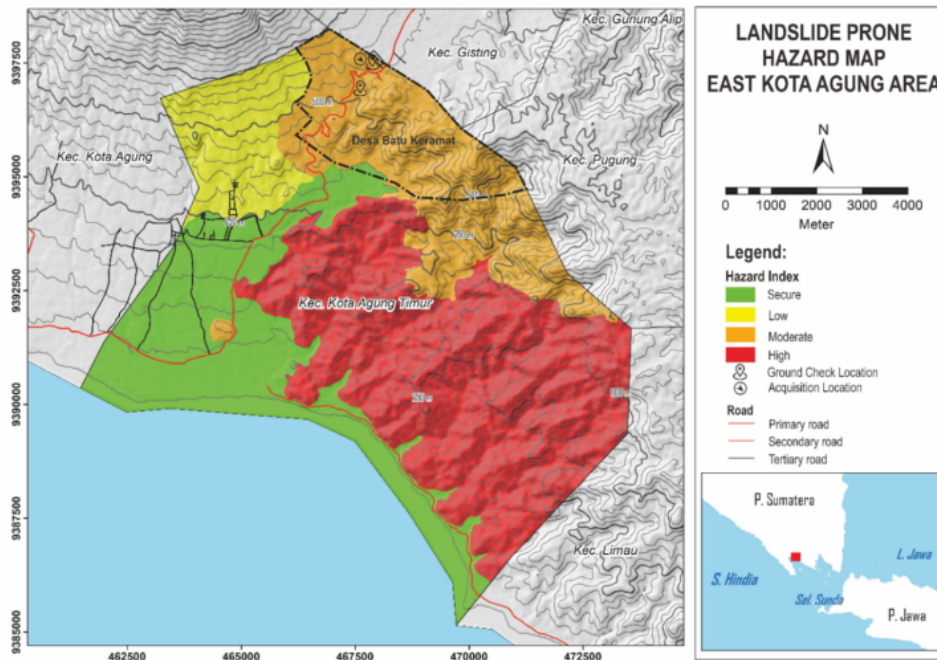
FIGURE 1. Landslide hazard map based on AHP method (4)-12] in East Kota Agung area and study area is located on the northern part with dash line border with acquisition location symbol (both of SfM and ERT). The research area is included in the moderate category, and it is proven that landslides occur in several areas.
