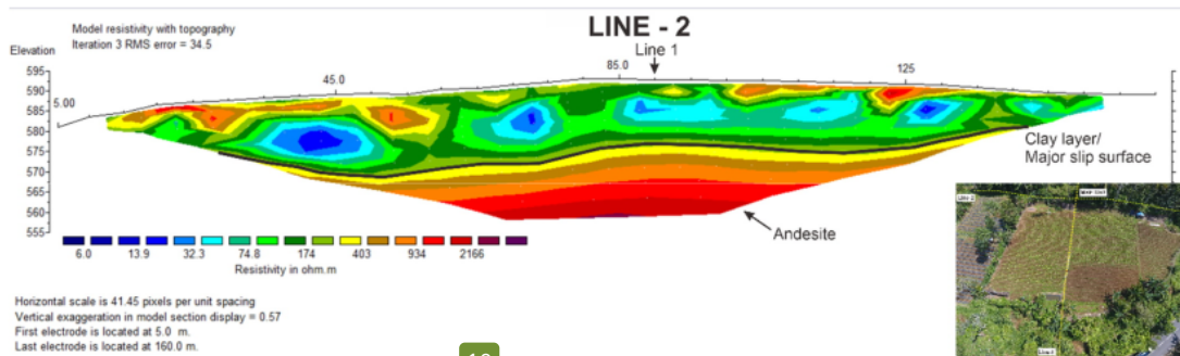
10 FIGURE 6. 2D ERT line-2 section of the research area using a Wenner-Schlumberger configuration.
