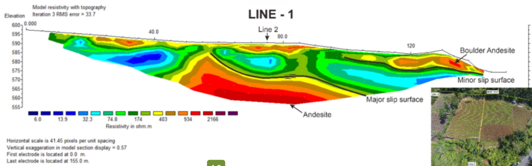
10 FIGURE 5. 2D ERT line-1 section of the research area using a Wenner-Schlumberger configuration.
