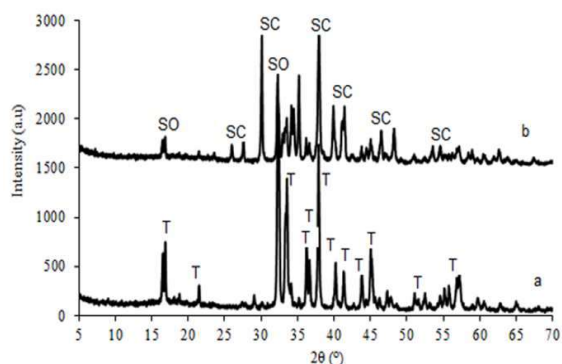
Figure 4. The x-ray Diffraction Patterns of the Original Sample (a) and the Sintered Sample (b) T= Thermonatrite (Na 2 CO 3 .H 2 O), SC= Sodium Carbonate (Na 2 CO 3 ), and SO= Sodium Oxide (Na 2 O)
