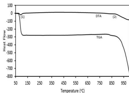
Figure 7. Analysis Thermal of \text{Na}_2\text{CO}_3
