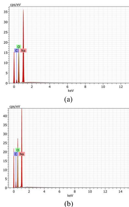
Figure 6. The EDS Spectra of Na 2 CO 3 Prepared at Different Concentrations of NaOH (a) 7.0 M and (b) 7.5 M
