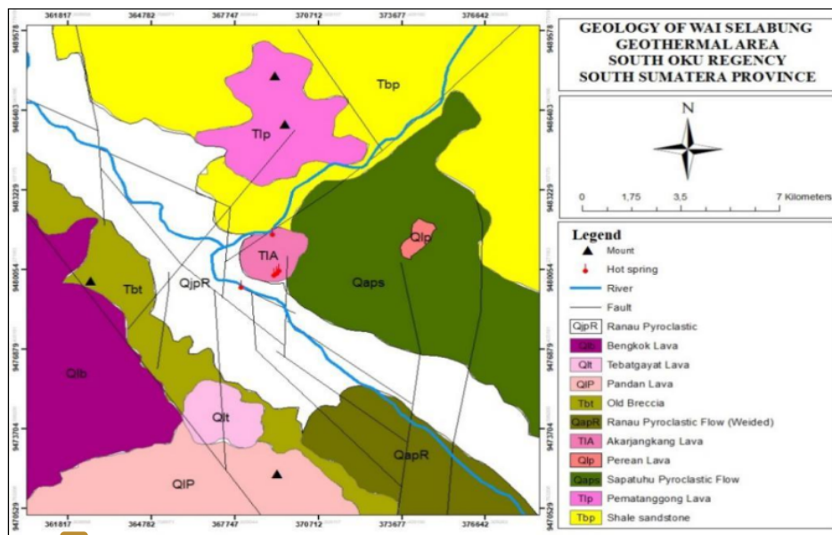
30 Figure 1. Geological map of the Wai Selabung geothermal area (modified from PSDG, 2011)
