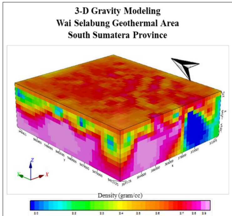
Figure 9. 3-Dimensional Model of the Research Area
