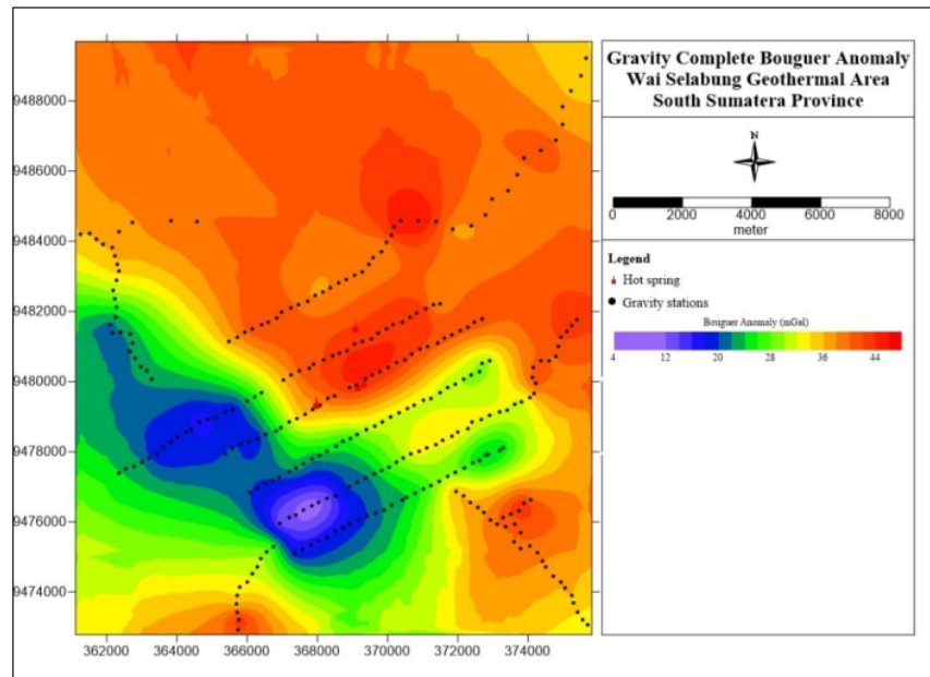
Figure 4. Bouguer Anomaly Map of the Study Area
