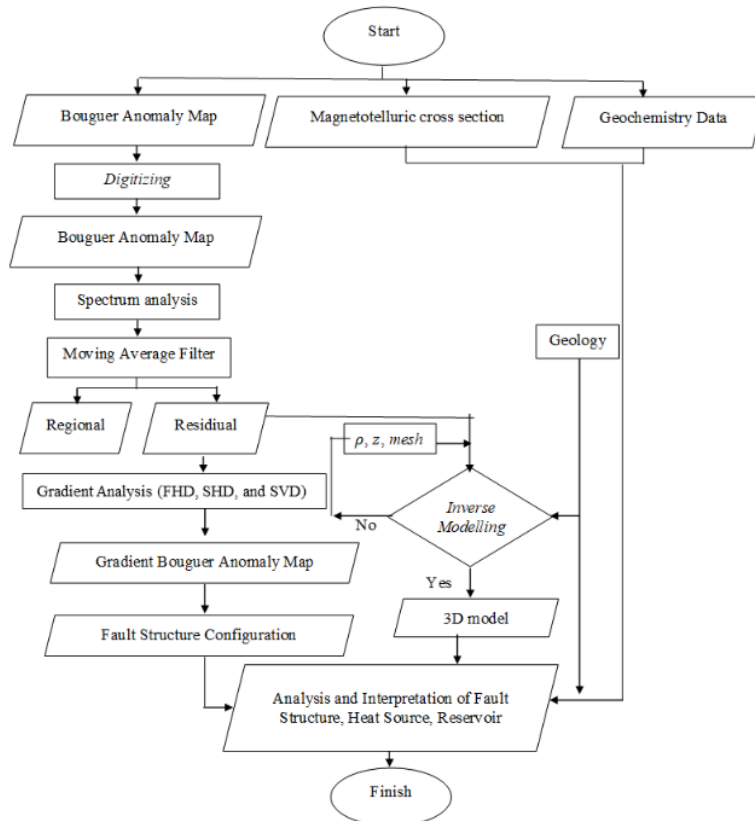
Figure 3. Flowchart of the Wai Selabung Geothermal Reservoir
