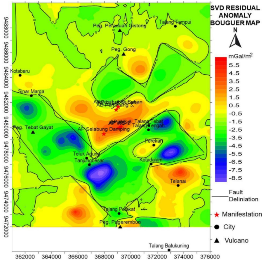
Figure 6. SVD Residual Anomaly Bouguer Map
