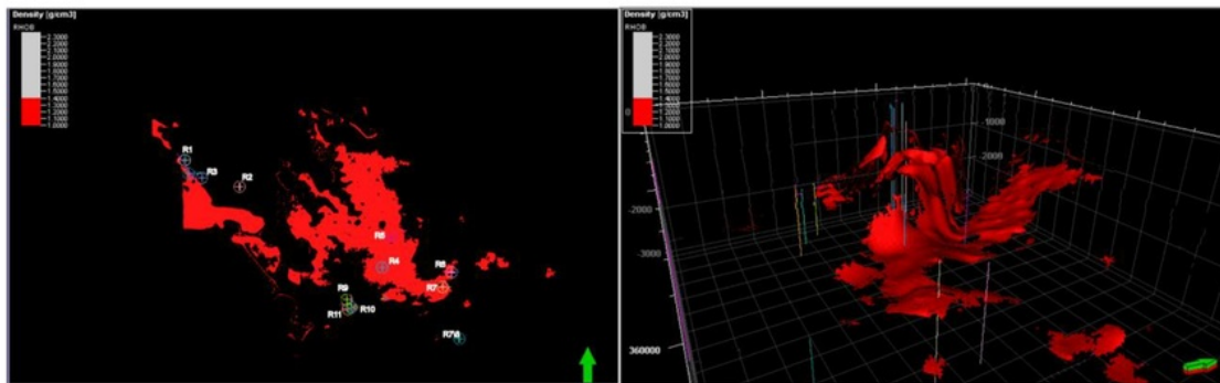
FIGURE 7. Coal seam A distribution from relative density cut-off 1.4 gr/cc
