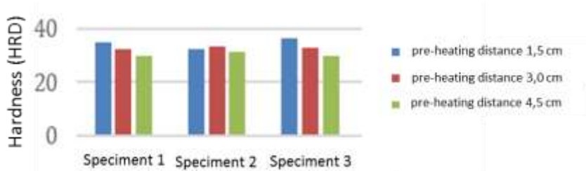
Figure 11. Hardness test graph
