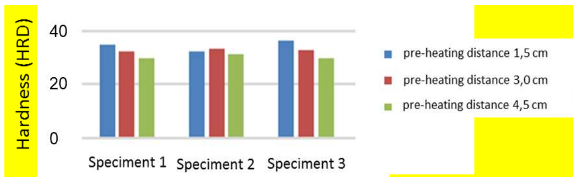
Figure 8. Hardness test results
