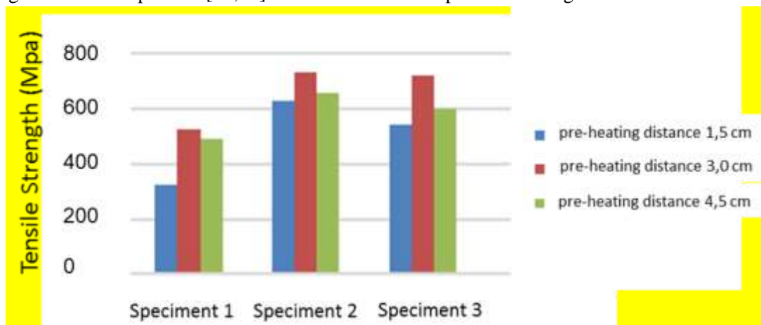
Figure 7. Tensile test results of the pre-heating specimens
