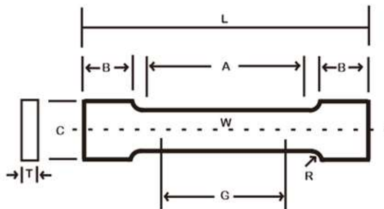
Figure 2. Tensile Testing Specimen Size ASTM E8.
