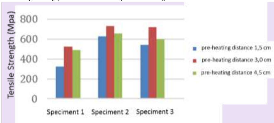
Figure 7. Tensile test results of the pre-heating specimens
