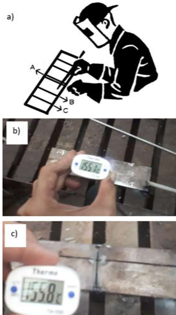
Figure 3. Illustration of the pre-heating process (a), with the distance of 1.5 cm (b) and 3 cm (c)
