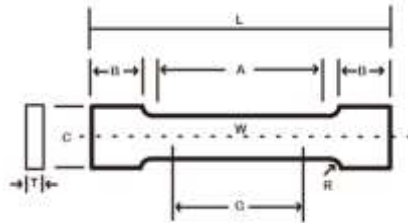
Figure 2. Tensile Testing Specimen Size ASTM E8.
