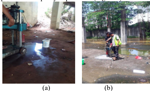
Figure 1. Basement condition: (a) protected, (b) unprotected
