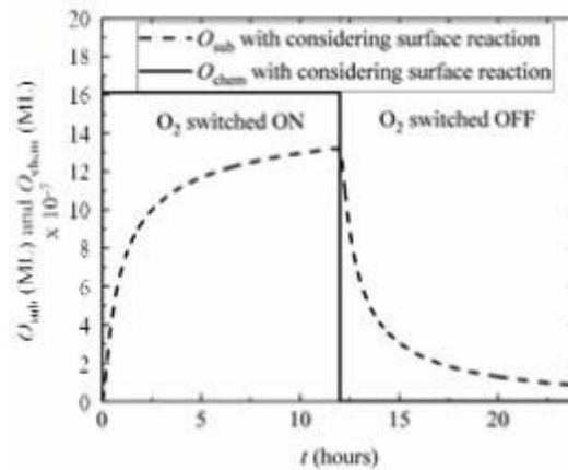
Figure 7. Chemisorbed and subsurface oxygen on Pt surface with RH = 42\% at room temperature ( 30^\circ C ) in synthetic air (consists of 80% of N_2 and 20% of O_2 , exposed by 1 atm of synthetic air for the first 12 hours and in vacuum condition for the last 12 hours, by considering the surface reaction but using only 10% of desorption energy of 2O^{(s)} on Pt.
