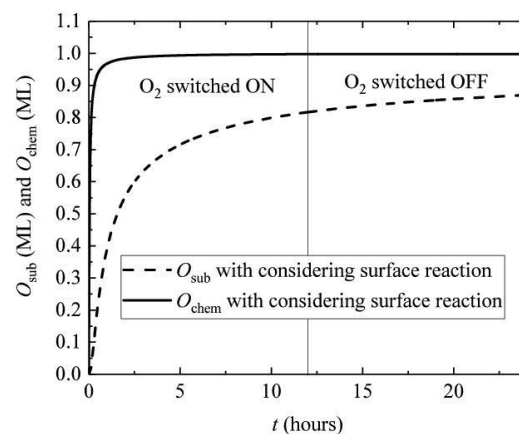
Figure 6. Chemisorbed and subsurface oxygen on Pt surface with RH = 42\% at room temperature ( 30^\circ\text{C} ) in synthetic air (consists of 80% of \text{N}_2 and 20% of \text{O}_2 ), exposed by 1 atm of synthetic air for the first 12 hours and in vacuum condition for the last 12 hours, by considering the surface reaction.
