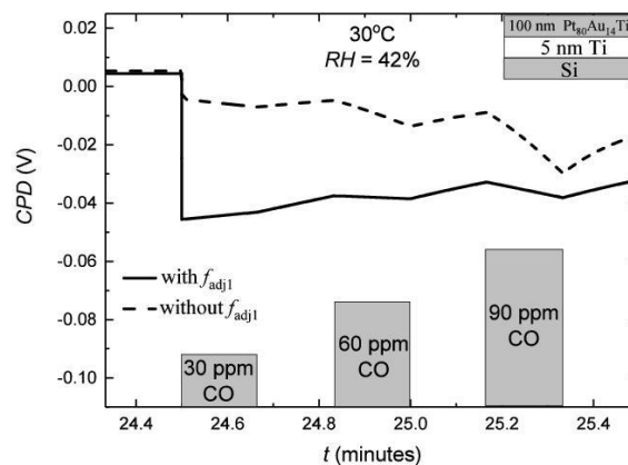
Figure 10. Simulation of loss signal phenomenon with and without SA on Pt_{80}Au_{14}Ti_6
