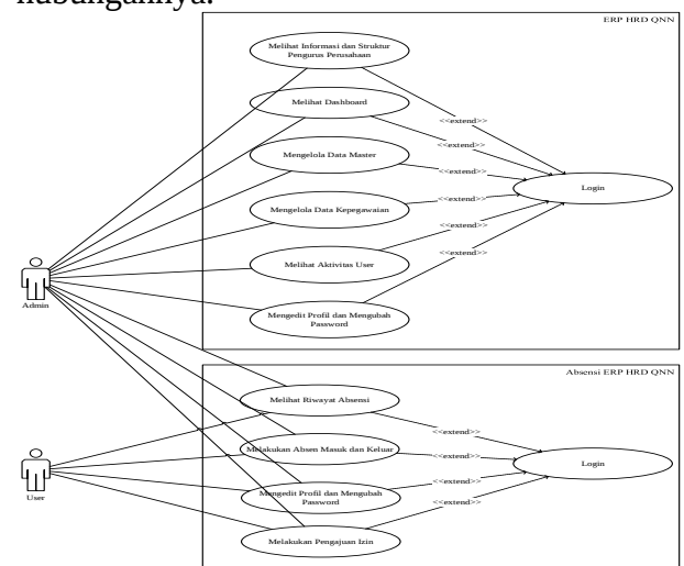
Gbr. 2 Use Case Diagram
