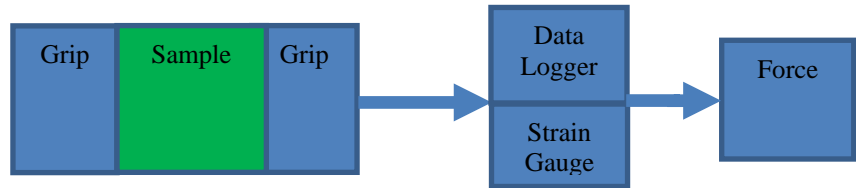
Fig. 2. Tensile strength test
