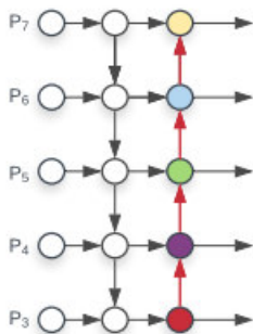
Fig. 3. PANet [9]
