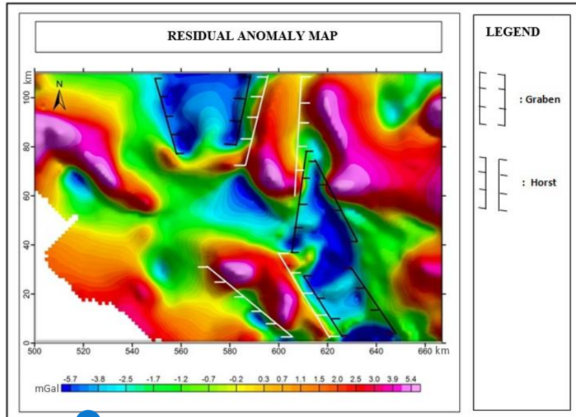
1 Figure 5. Residual anomaly map of the research area.
