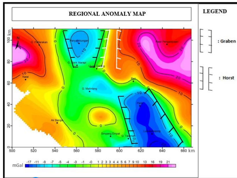
1 Figure 4. Regional anomaly map of the research area.
