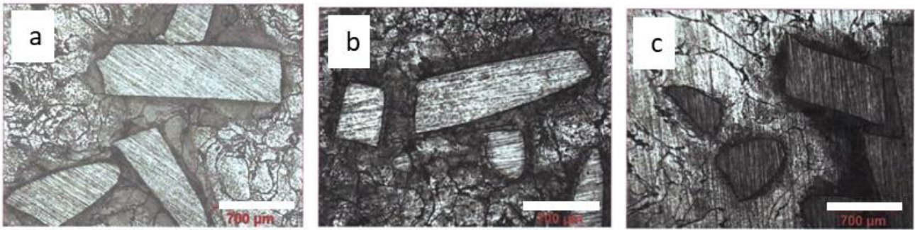
Figure 7. Structure of Micro-Specimen (a). P-Mg 100 µm, P-Mg 200 µm and (c). P-Mg 250 µm
