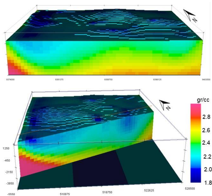
Figure 7. The subsurface density distribution model results from the 3D inversion modeling of the Bouguer anomaly in the Way Ratai geothermal area
