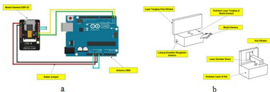
Fig 1. a) Electronic Circuit b) Body Props
