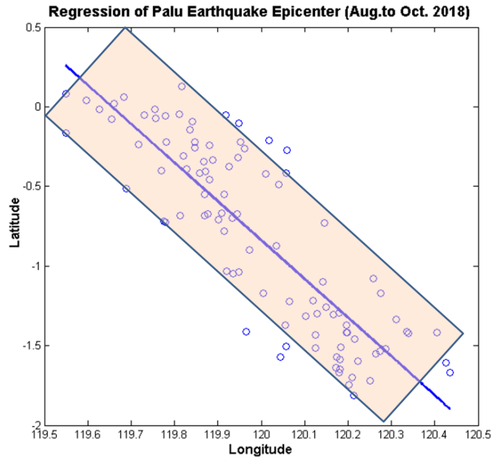
Figure 8. Estimated of line fracture of the Palu earthquake in August to October 2018.
