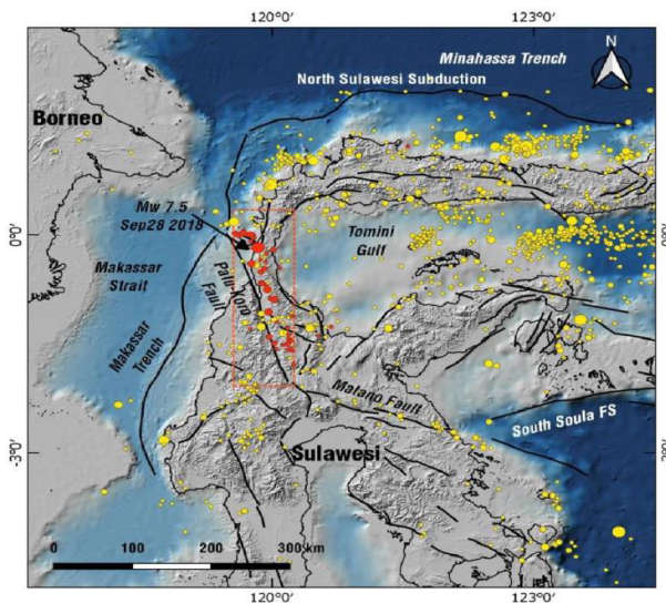
Figure 3. Tectonic setting and seismicity of Sulawesi, Indonesia [7].
