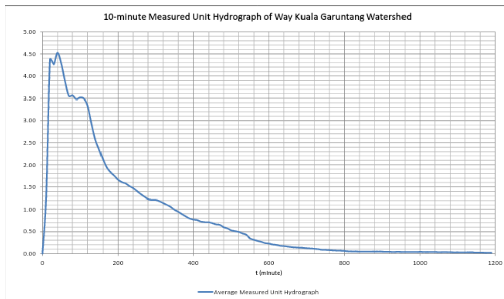
Figure 6. Average IUH for 5 flood events
