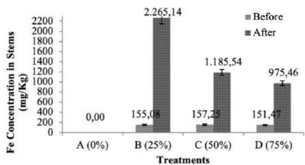
Figure 5. Fe Concentration in the stems of water hyacinths before and after treatments
