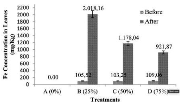
Figure 6. Fe Concentration in the leaves of water hyacinths before and after treatments
