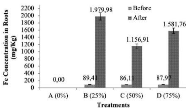
Figure 4. Fe Concentration in the roots of water hyacinths before and after treatments
