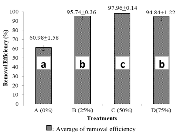
Figure 3. Percentage averages of Fe concentration decrease in the water base on the treatments. Notes: a, b, c, d: Different letters indicate significant differences. Treatments B (25% coverage of water hyacinths) and D (75% coverage of water hyacinths) showed no significant difference
