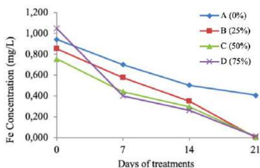
Figure 1. Decreased concentration of Fe in water for 21 days of treatment
