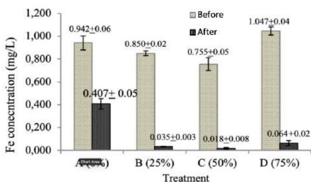
Figure 2. Fe concentration in the water before and after treatments
