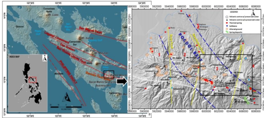
27 Fig. 1. Map of the study area location and faults structure in the Bac-Man geothermal field [2, 3]
