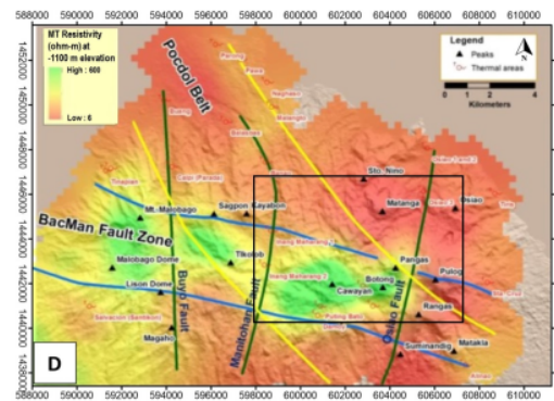
Fig. 3. An iso-resistivity map at a depth of -1100\text{ m} from MSL which is correlated with the geological structure in the area, shows that the central part of the Bac-Man fault zone has a low resistivity value [3]
