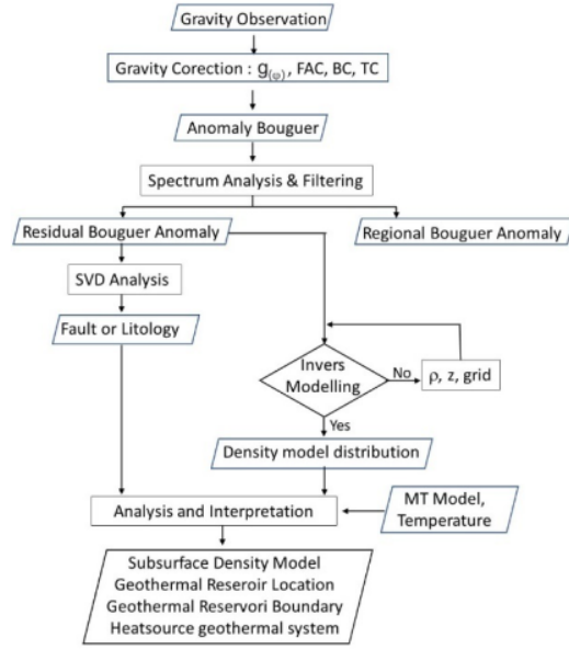
Fig. 5. Flowchart of research in determining the boundary of a geothermal reservoir
