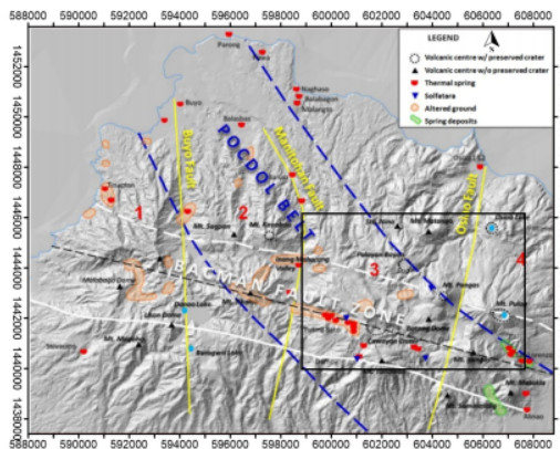
Fig. 2. Structure and manifestations at the Bac-Man geothermal field [2]
