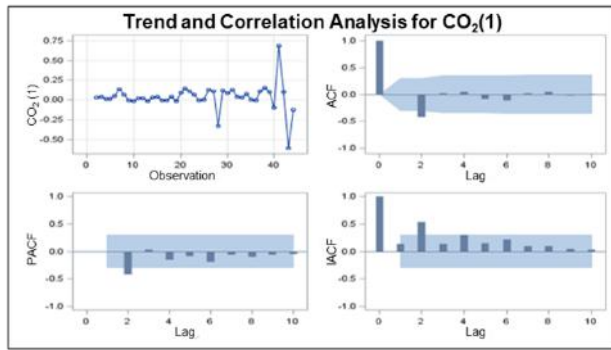
1 Figure 5. Trend and Correlation Analysis of CO 2 after Differencing, d=1
