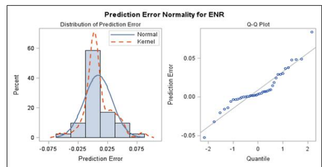
Figure 6. Prediction Error Normality for Energy (ENR)
