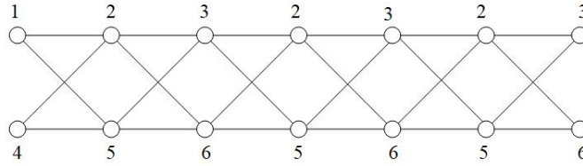
Figure 1. A locating coloring of D_2(P_7) .
