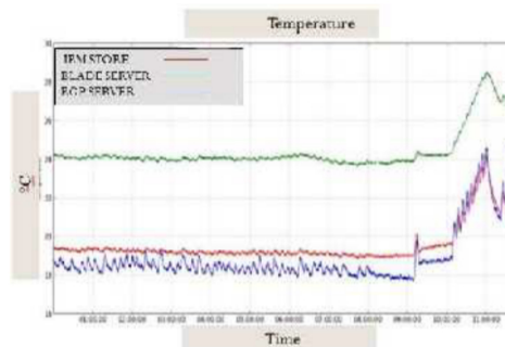
Fig 8. Temperature Report
