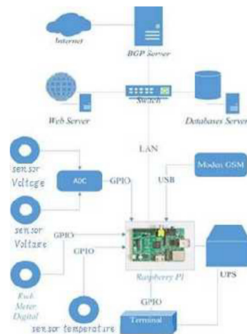
Fig 2. Hardware Design Architecture
