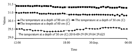
Fig. 10: Real-time temperature monitoring (Anak Krakatoa volcano)
