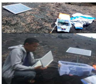
Fig. 9: Set-up the device nearby the seismograph station
