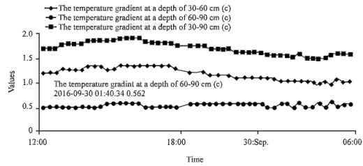
Fig. 11: Real-time gradient temperature (Anak Krakatoa volcano)
