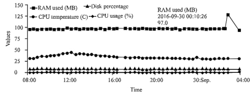
Fig. 12: Real-time the performance monitoring of single board computer BCM2835
