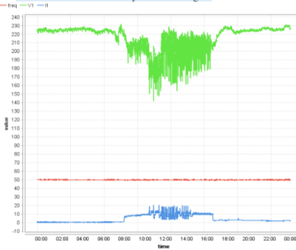
Fig. 16: Electrical Quantities Measurement on Phase 1 for 1 day
