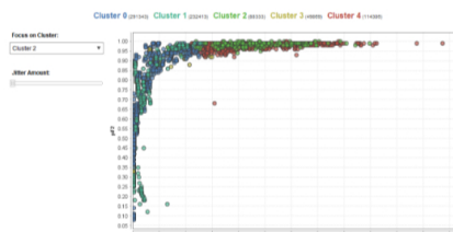
Scatter plot relation between I2 and pF2 on Phase 2
