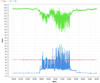
Fig. 11: Electrical Quantities Measurement on Phase 0 for 1 day
