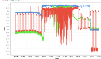
(b) Power Factor value on all Phase
