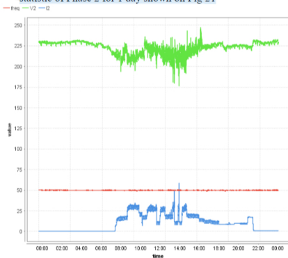
Fig. 21: Electrical Quantities Measurement on Phase 2 for 1 day
