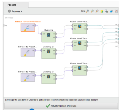
Fig. 6: Process of models and operator creation for clustering analysis on RapidMiner
