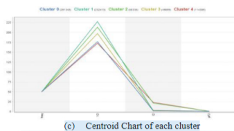
Fig. 18: (a) (b) (c) Cluster Data Visualization of Phase-2
