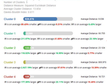
Fig. 14: Phase 1 data cluster overview
