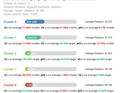
Fig. 19: Phase 2 data cluster overview
