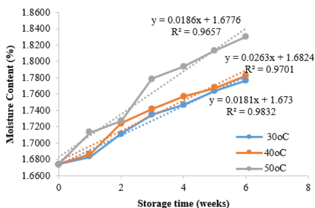
Figure 1. Linear regression of order 0 of moisture content in instant chocolate vacuum packaged using PP plastic
