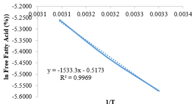
Figure 6. Graph of the relationship between 1/T value with \ln k instant chocolate FFA levels in PP vacuum packaging
