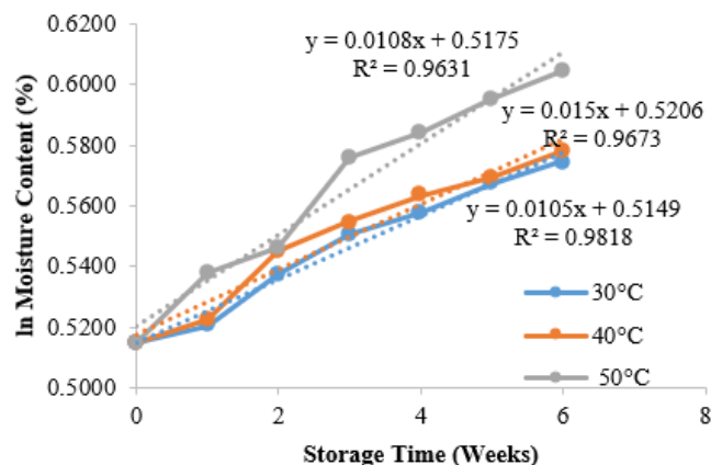
Figure 2. Order 1 linear regression of water content in instant chocolate vacuum packaged using PP plastic
