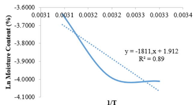
Figure 3. Graph of the relationship between 1/T value with \ln k of moisture content in instant chocolate vacuum packaged with PP plastic
