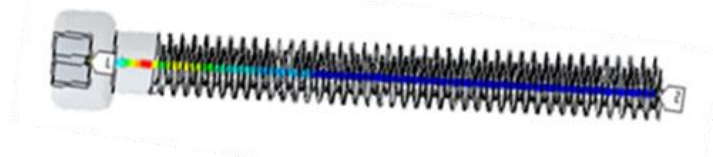
Fig. 10. Linearized equivalent stress bone screws pullout
