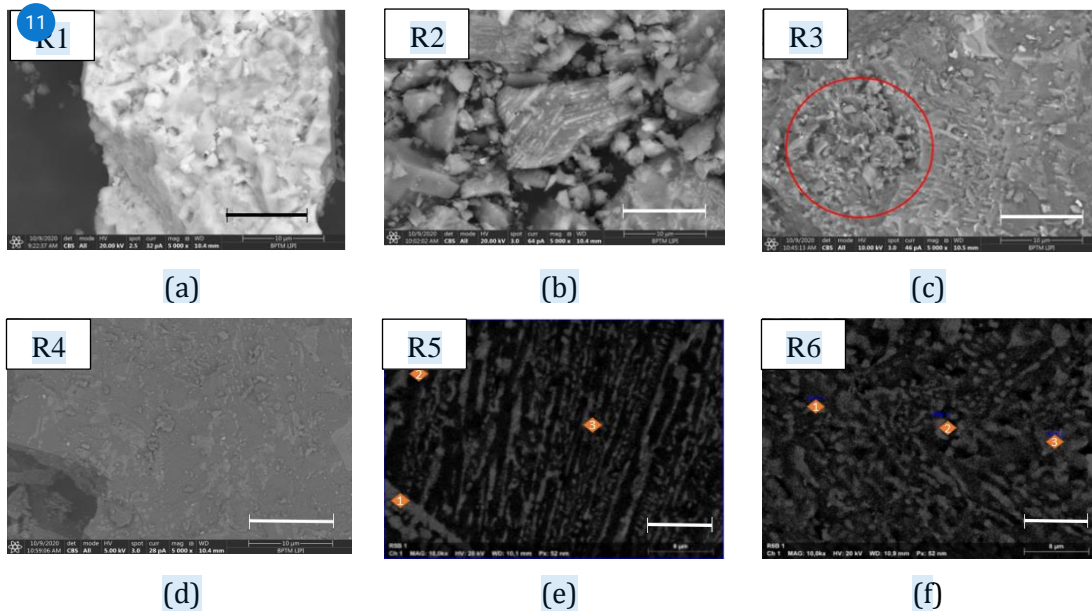
Figure 5 Scanning electron microscopy of G.C.s obtained at: (a) 850°C-3hrs; (b) 950°C-3hrs; (c) 1,050°C-3hrs; (d) 850°C-8hrs; (e) 950°C-8hrs; and (f) 1,050°C-8hrs. Bars were 10μm.
