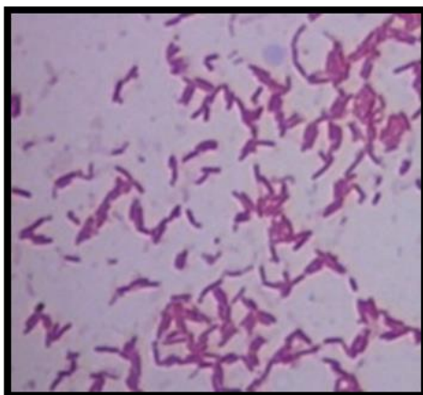
Figur 3 Gram staining
