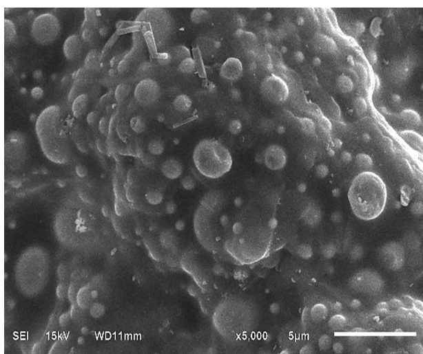
Figure 3. Scanning Electron Micrograph of the Ag/SiO 2 composites with different Ag concentrations at a sintering temperature of 850 °C: a) 0.3 M, b) 0.5 M, and c) 0.8 M (magnification 5 kX).
