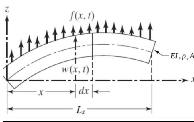
Figure 8. Continuous beam [22]
