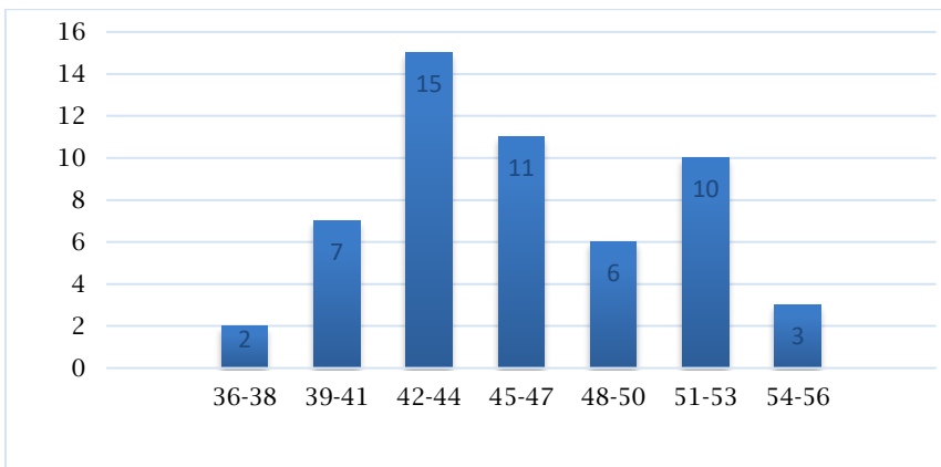
Figure 2. The histogram of the X_1 frequency distribution
