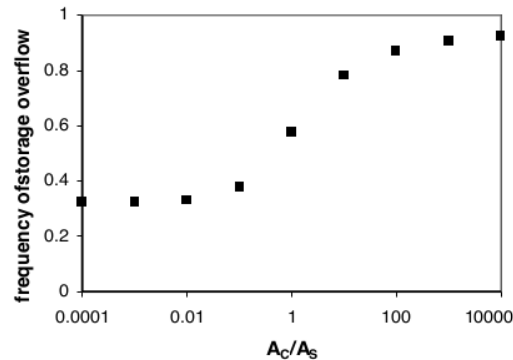
Figure 1. Frequency of Storage Overflow
