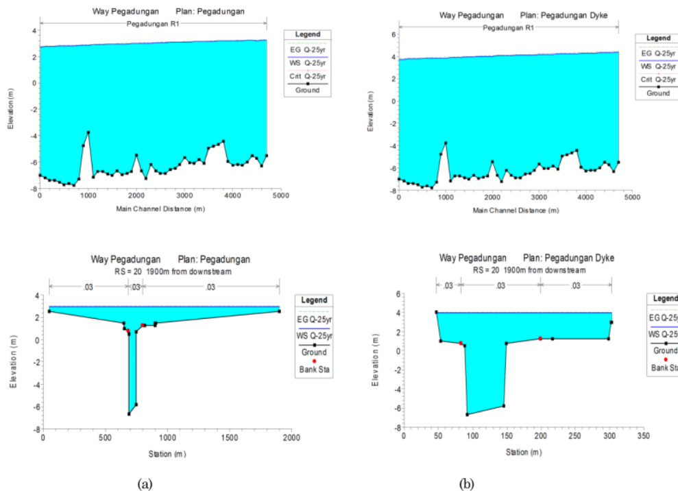
Figure 3. Water Surface for Long Profiles (top figures) and Cross Sections (bottom figures) in the Simulation at Existing Condition or without Dyke (a) and with Dyke (b)
