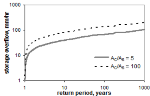
Figure 2. Flood Frequency Curve of Storage Overflow
