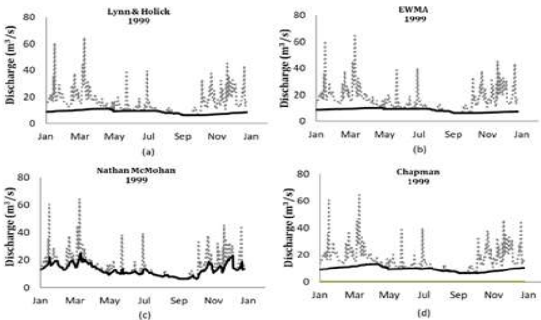
Figure 2. Illustration of total discharge and baseflow hydrographs using RDF methods: (a) Lynn & Holick, (b) EWMA, (c) Nathan McMohan, and (d) Chapman.
