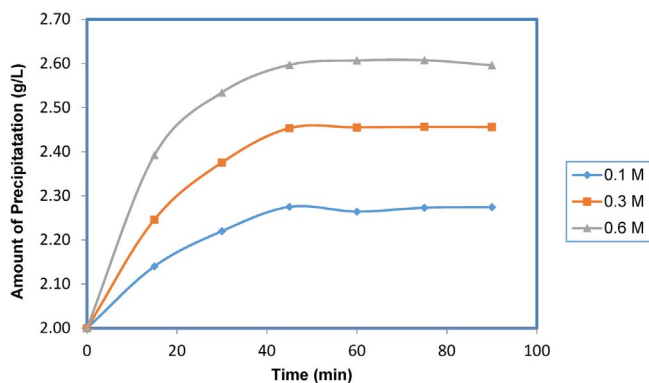
Fig. 2. The growth rate of \text{CaCO}_3 precipitation at various growth solution concentration.
