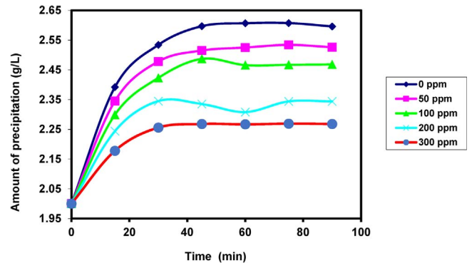
Fig. 5. Effect of inhibitor added on the formation of \text{CaCO}_3 precipitation at the growth solution concentration of 0.6 M.
