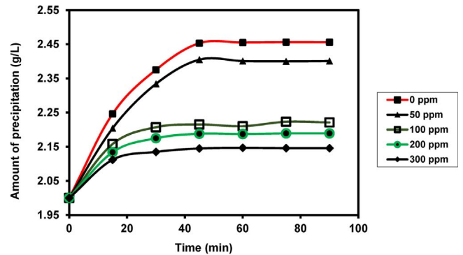
Fig. 4. Effect of inhibitor added on the formation of \text{CaCO}_3 precipitation at the growth solution concentration of 0.3 M.
