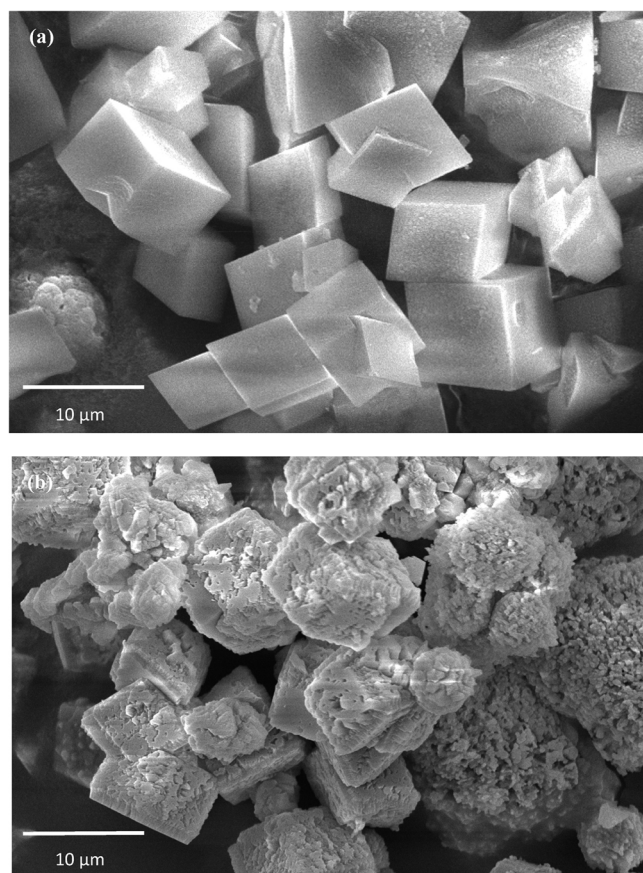
Fig. 7. Morphology of \text{CaCO}_3 crystals (a) in the absence of inhibitor (b) in the presence of inhibitor 300 ppm at the concentration of growth solution of 0.6 M (Magnification 2500 \times ).
